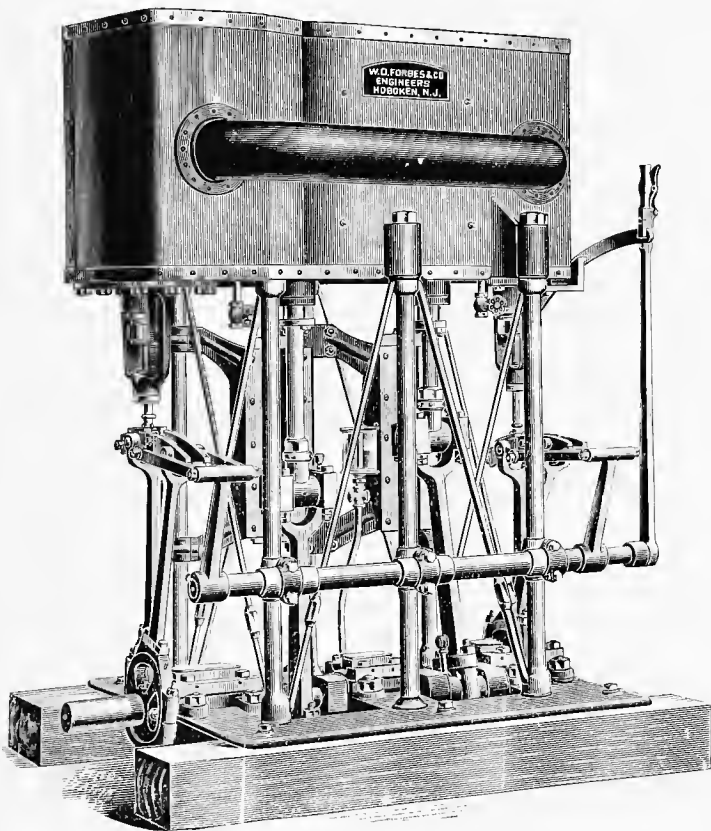
FORBES' VERTICAL YACHT ENGINE.—By W. D. Forbes & Co.
